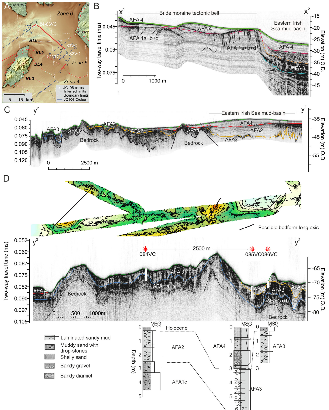
Figure 10. Sea floor acoustic and stratigraphical data from east and north of the Isle of Man. (A) The location, zones and boundary limits, the JC106 cruise track (green), the JC106 cores and transect lines x^1-x^2 , y^1-y^2 and y^2-y^3 . (B) East of the Isle of Man line x^1-x^2 the sub-bottom profiler data traverse the glaciotectonic axis of the Bride Moraine. (C) Line y^1-y^2 the sub-bottom profiler data extend from the eastern Irish Sea mud basin to the Solway Firth. (D) Planform multi-beam data with 2-m contour intervals, sub-bottom profiler data and the vibrocore stratigraphy from line y^2-y^3 in the Solway Firth. The sub-bottom profiler data are annotated with acoustic facies (Table 6), boundaries and core locations. [Colour figure can be viewed at wileyonlinelibrary.com ]
