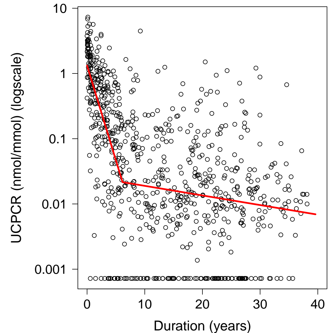
Age at diagnosis > 10.8y
