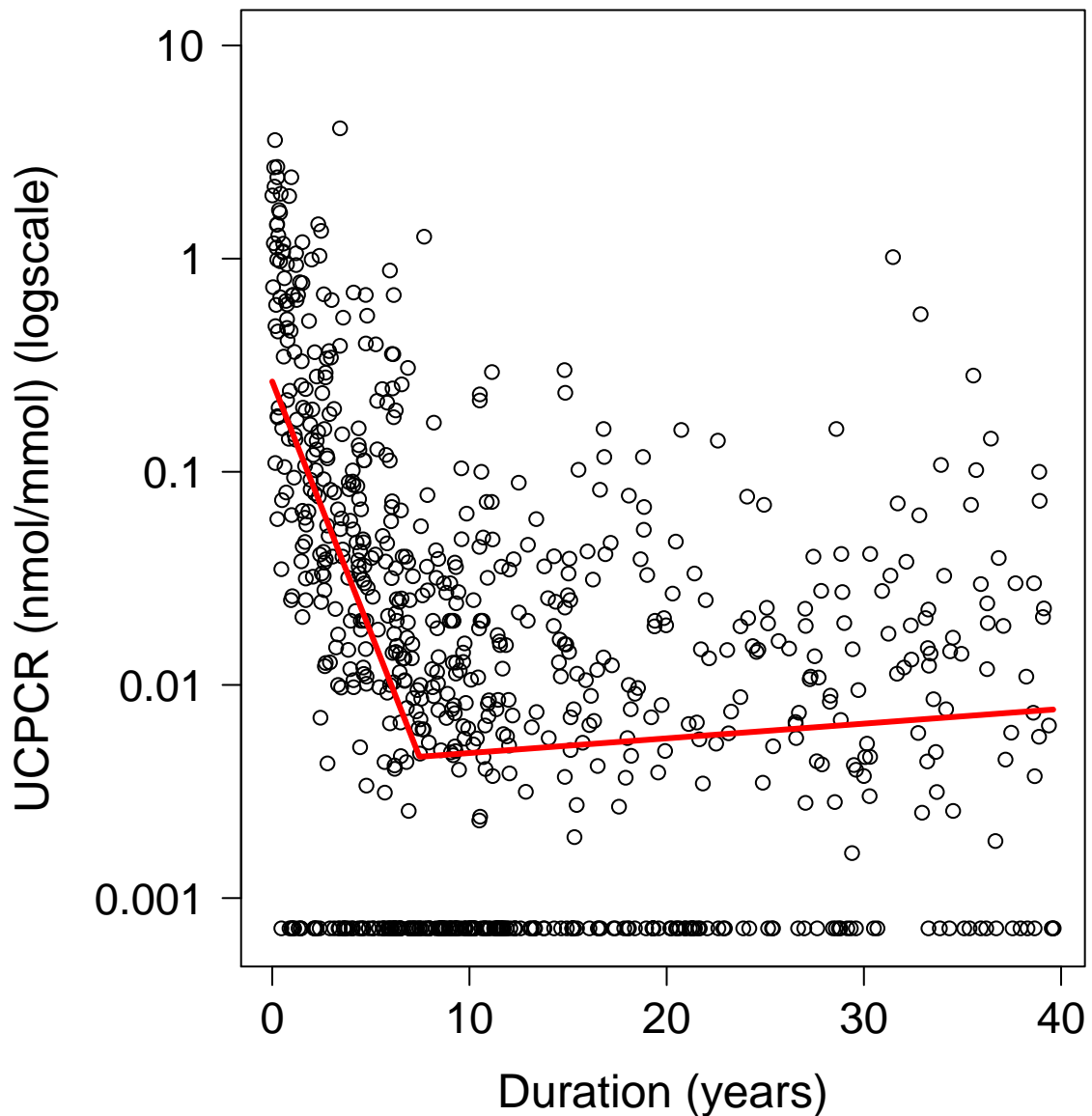
Age at diagnosis \leq 10.8y
