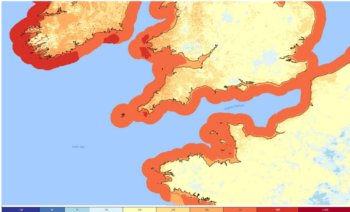
Figure 3-7: Aggregated mean wind power density ( W/m^2 ) at 50m in the southern UK and northern France (source: Global Wind Atlas, 2017).
