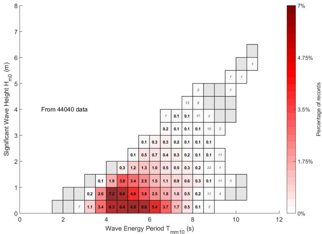
Figure 3-5: Scatter diagram showing the relationship between significant wave height and energy period at the FaBTest wave energy test site, produced by University of Exeter (Parish & Hardwick 2012).
