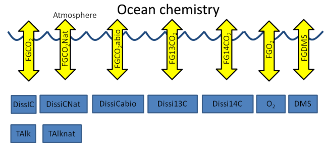
Figure 16. Ocean chemistry including the suite of carbon system tracers and those undergoing gas exchange.
